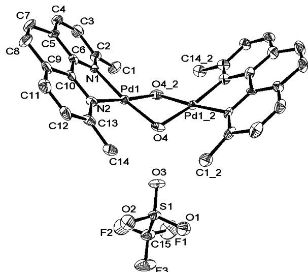
Figure 2. Solid-state structure of 4 on a crystallographic 2-fold axis with ellipsoids drawn at the 50% probability level. Hydrogen atoms, except those corresponding to the \mu -OH groups, and one triflate anion are omitted for clarity. Selected bond lengths ( \text{\AA} ) and angles (deg): Pd1–N1, 2.038(8); Pd1–N2, 2.047(9); Pd1–O4, 2.014(9); Pd1–O4_2, 2.006(9); O4–Pd1–O4_2, 79.3(3); N1–Pd1–N2, 82.1(3); Pd1–O4_2–Pd1_2, 95.8(3); C14–C13–N2–Pd1, 14.4(3); C1–C2–N1–Pd1, 12.5(5). Nonbonded distances ( \text{\AA} ): Pd1–Pd1_2, 2.982(2); O4–O4_2, 2.564(9); C(methyl)–Pd1, 3.44(8) (average); C(methyl)–( \mu -O), 2.89(3) (average); O3–O4, 2.74(9).
